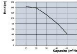
Performans Eğrisi 9LD925-2 R 526
