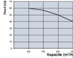
Performans Eğrisi LDW2204 NM 80-200
